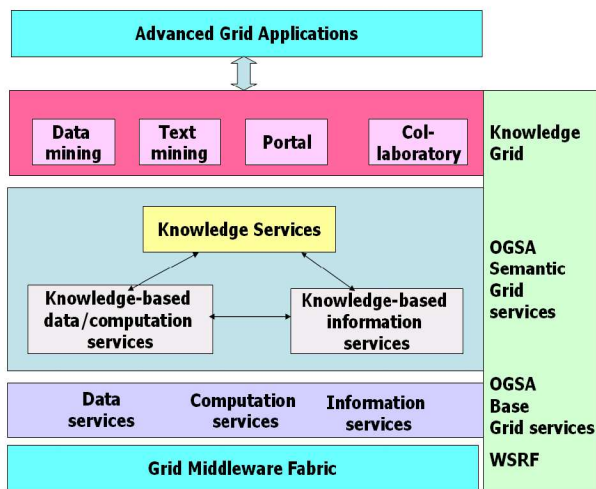
Fig. 2 The Semantic/Knowledge Grid Stack
