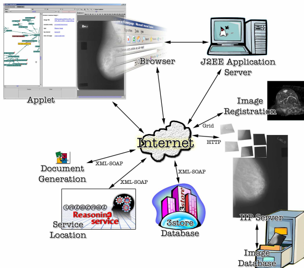
Figure 2 MIAKT Mixed Web and Grid Services Architecture
