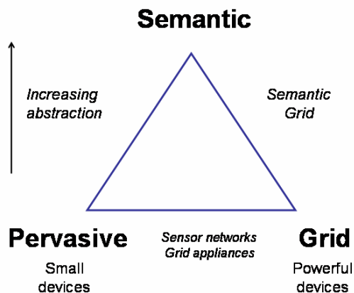
Figure 4 The Semantic-Pervasive-Grid triangle
