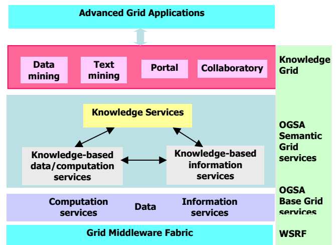
Figure 3 Semantic Grid Architecture (due to Goble et al)
